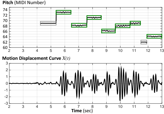
Figure 5. Pitch trajectory with detected vibrato notes marked by green rectangles from audio analysis and the left-hand motion curve of the corresponding player from video analysis.
