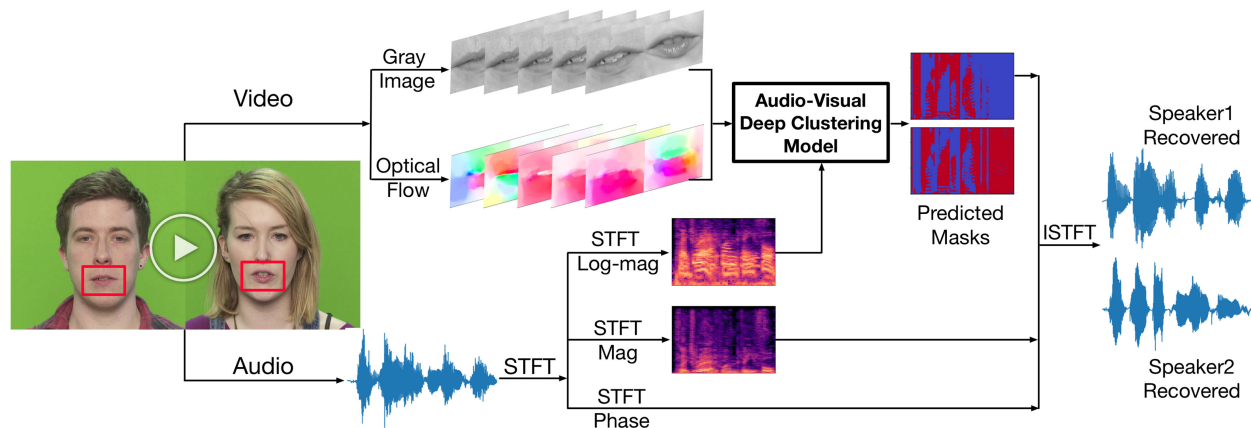
Fig. 1. Proposed audio-visual separation system: The Audio-Visual Deep Clustering (AVDC) model integrates both appearance (gray image) and motion (optical flow) information of the lip regions with the log magnitude spectrogram of the audio mixture to predict masks of source spectrograms. These masks are then applied to the complex spectrogram of the audio mixture followed by inverse-STFT for separation.
