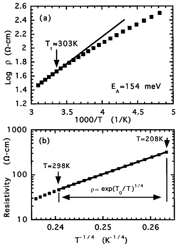
FIG. 4. (a) Arrhenius plot of resistivity for sample f , \text{YBa}_2\text{Cu}_3\text{O}_{6.3} . Above approximately 300 K, the conduction shows thermally activated behavior with E_A \approx 154 meV. Below 300 K, the local activation energy decreases monotonically. (b) Plotting the natural log of the resistivity vs T^{-1/4} shows a linear relationship below 300 K. This \exp(T^{-1/4}) temperature dependence below 300 K is consistent with Mott's variable range hopping model.
