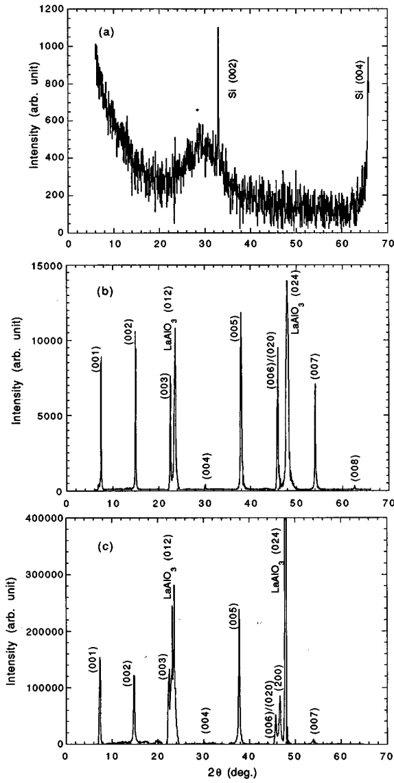
FIG. 2. (a) Typical x-ray diffraction pattern of amorphous Y-Ba-Cu-O thin films. Position marked * could be due to the presence of the Y_2BaCuO_5 phase. (b) XRD pattern for sample f , a single crystal tetragonal YBa_2Cu_3O_{6+x} ( x \sim 0.5 ) thin film on LaAlO_3 substrate. (c) XRD pattern for sample g , a single crystal tetragonal YBa_2Cu_3O_{6+x} ( x \sim 0.3 ) thin film on LaAlO_3 substrate.
