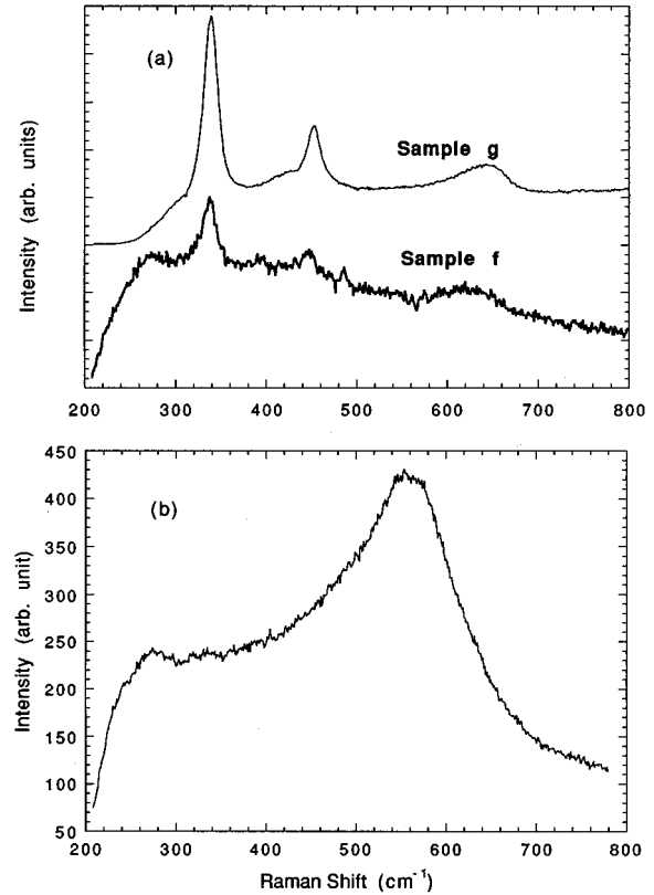
FIG. 3. Raman spectra for Y-Ba-Cu-O samples at room temperature. (a) Spectra for the crystalline samples f and g . (b) A typical Raman spectrum for the amorphous Y-Ba-Cu-O thin films ( a-e ).
