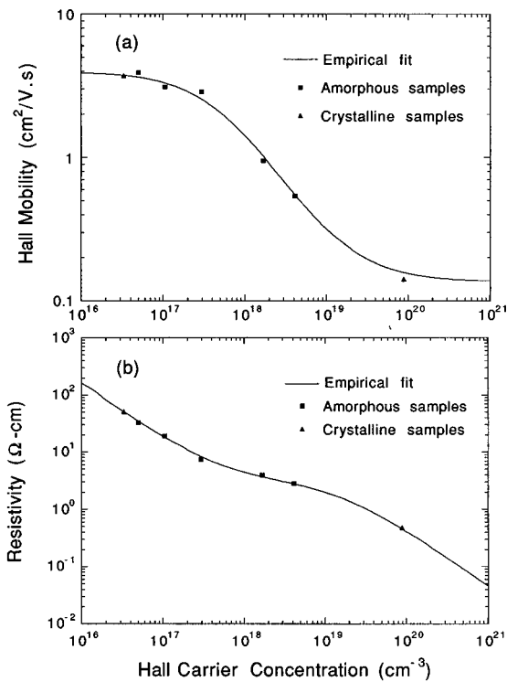
FIG. 5. (a) Hall mobility and (b) dc resistivity vs carrier concentration for the semiconducting thin films at T=295 K. The fitting constants for Eq. (3) were determined to be \mu_{\min}=0.135 cm 2 /V s, \mu_0=3.84 cm 2 /V s, and N_{\text{ref}}=5 \times 10^{17} cm -3 .
