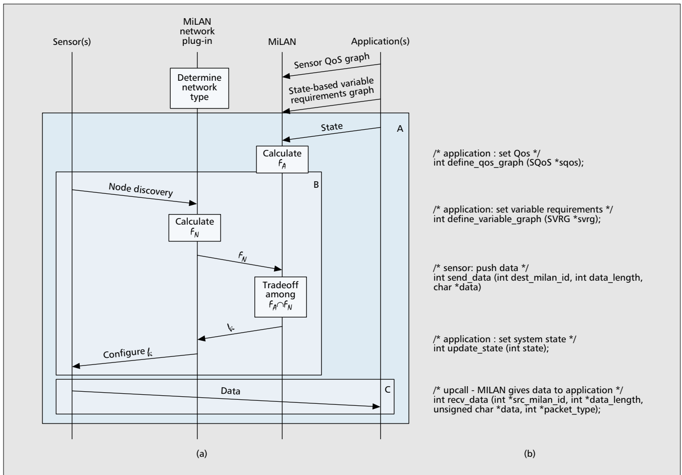
■ Figure 5. a) A high-level overview of MiLAN operation. Segment A repeats when the application changes its state based on data received from the sensors. Segment B repeats when sensors arrive in the network. Segment C repeats as data arrives from each sensor, and represents the normal operation of MiLAN conveying information from the sensors to the application. b) Partial MiLAN API. Applications represent their Sensor QoS graph to MiLAN using the SQoS structure and the define_qos_graph function, and they represent their State-based Variable Requirements graph to MiLAN using the SVRG structure and the define_variable_graph function. After initialization, sensors send data to the application using the send_data function and applications receive the data from MiLAN via an upcall from the recv_data function. Applications specify to MiLAN that they have changed state through the update_state function.
