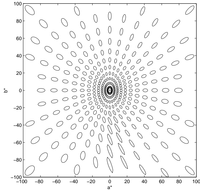
Figure 1: “Ellipses” corresponding to a CIEDE2000 color difference of \Delta E_{00} = 1.0 in the a^*-b^* plane.
